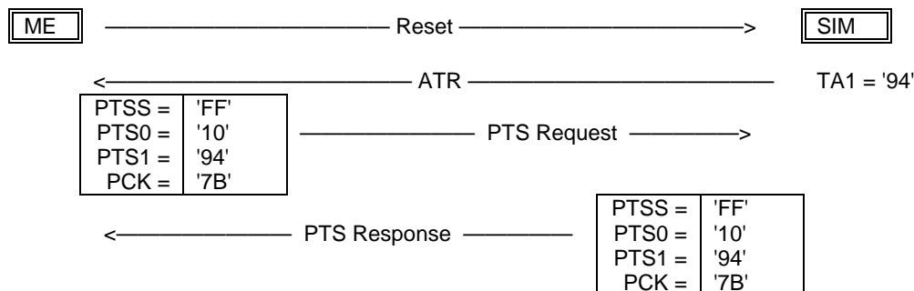
Figure 2: PTS procedure requesting enhanced speed values (F=512, D=8, see clause 5.8.3)
